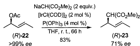
Scheme 8. Allylic substitution using a substrate with a potentially symmetric ( \pi -allyl)Ir III intermediate
