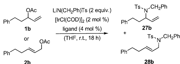
Scheme 9. Ir I -catalysed allylic amination of ( rac )- 1b and ( E )- 2b
