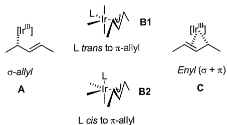
Figure 3. Possible intermediates in the allylic substitution of acetate ( R )- 22
