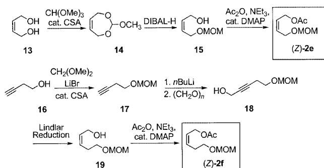
Scheme 5. Synthesis of substrates ( Z )- 2e and ( Z )- 2f (CSA: camphorsulfonic acid)
