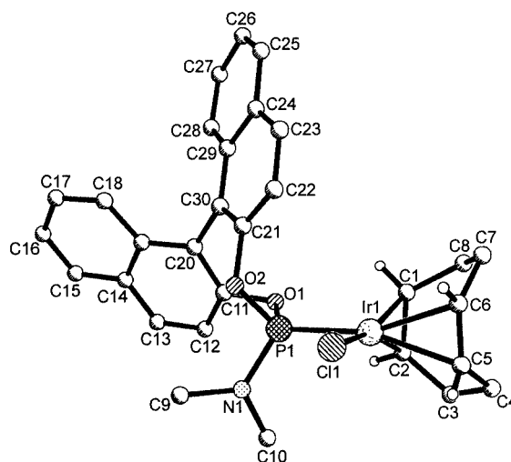
Figure 4. X-ray structure of complex 29 ; selected bond lengths (Å): Ir(1)–C(1) 2.114(6), Ir(1)–C(2) 2.118(6), Ir(1)–C(5) 2.222(5), Ir(1)–C(6) 2.222(5), Ir(1)–P(1) 2.2363(13), Ir(1)–Cl(1) 2.358(1), C(1)–C(2) 1.434(8), C(5)–C(6) 1.371(8)
