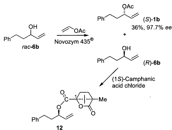
Scheme 4. Kinetic resolution of the alcohol 6b by enzyme-catalysed esterification and confirmation of the absolute configuration of the products
