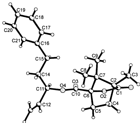
Figure 2. Crystal structure of ester 12 prepared by reaction of the enantiomerically pure alcohol ( R )- 6b with ( 1S )-camphanic acid chloride
