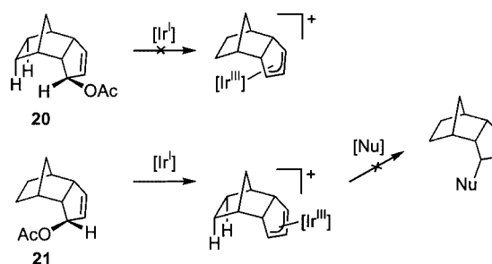
Scheme 7. Ir I -catalysed allylic substitutions
