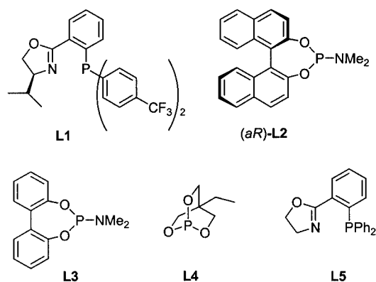
Figure 1. Ligands used in Ir I -catalysed substitutions
