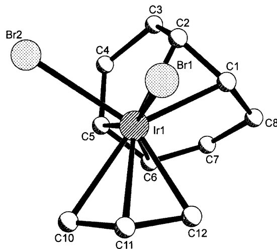
Figure 6. Crystal structure of complex 31 ; selected bond lengths (Å) with estimated standard deviations: Ir(1)–C(10) 2.321(8), Ir(1)–C(11) 2.241(9), Ir(1)–C(12) 2.176(8), C(10)–C(11) 1.36(1), C(11)–C(12) 1.46(1), C(1)–C(2) 1.39(1), C(3)–C(4) 1.53(1), C(5)–C(6) 1.38(1), C(7)–C(8) 1.53(1)
