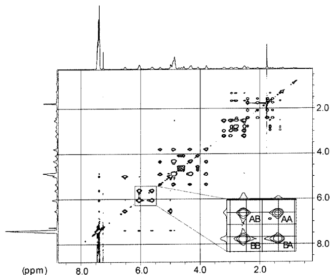
Figure 7. 1 H- 1 H EXSY spectrum of complex 30 recorded at –40 °C (CDCl 3 , 500.13 MHz); cross peaks chosen for the calculations are enlarged; A and B denote the minor and major isomer, respectively
