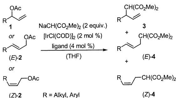
Scheme 1. General scheme for the Ir I -catalysed allylic alkylation of monosubstituted allylic acetates
