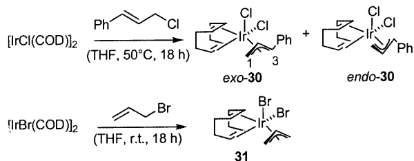
Scheme 10. Oxidative addition of allyl halides to Ir I complexes
