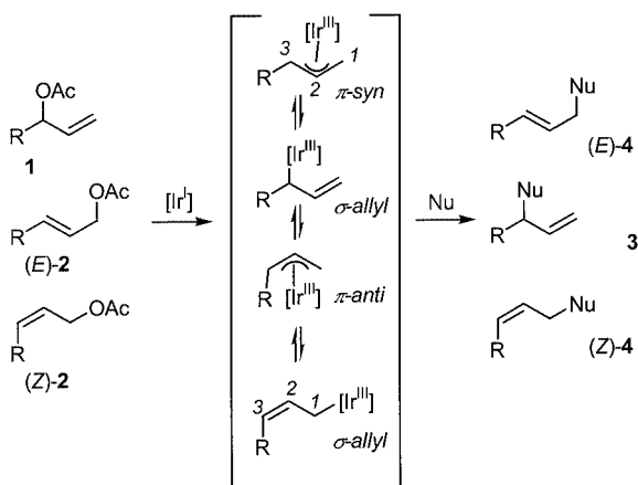
Scheme 6. Ir I -catalysed allylic substitution of substrates 1 and 2 via \sigma - and \pi -allyl intermediates
