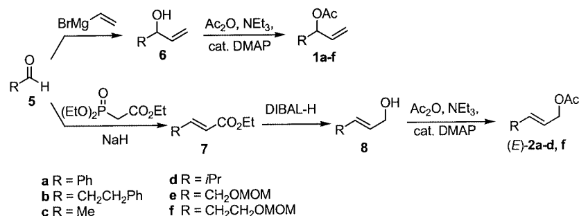
Scheme 2. Synthesis of substrates 1 and ( E )- 2 ; DIBAL-H: Diisobutylaluminium hydride; DMAP: 4-dimethylaminopyridine
