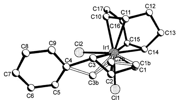
Figure 5. Crystal structure of complex 30 ; selected bond lengths (Å) with estimated standard deviations: Ir(1)–C(1)/C(1B) 2.11(3)/2.31(5), Ir(1)–C(2)/C(2B) 2.24(2)/2.31(2), Ir(1)–C(3)/C(3B) 2.45(1)/2.48(1), C(1)–C(2) = 1.44(1), C(1B)–C(2B) 1.44(2), C(2)–C(3) 1.35(1), C(2B)–C(3B) 1.34(2)
