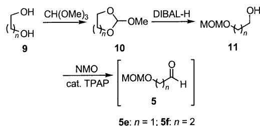
Scheme 3. Synthesis of aldehydes 5 ; TPAP: ( n Pr 4 N)[RuO 4 ]; MOM: methoxymethyl; DMAP: 4-dimethylaminopyridine; NMO: N -methylmorpholine N -oxide
